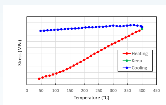
Temp/Stress data
